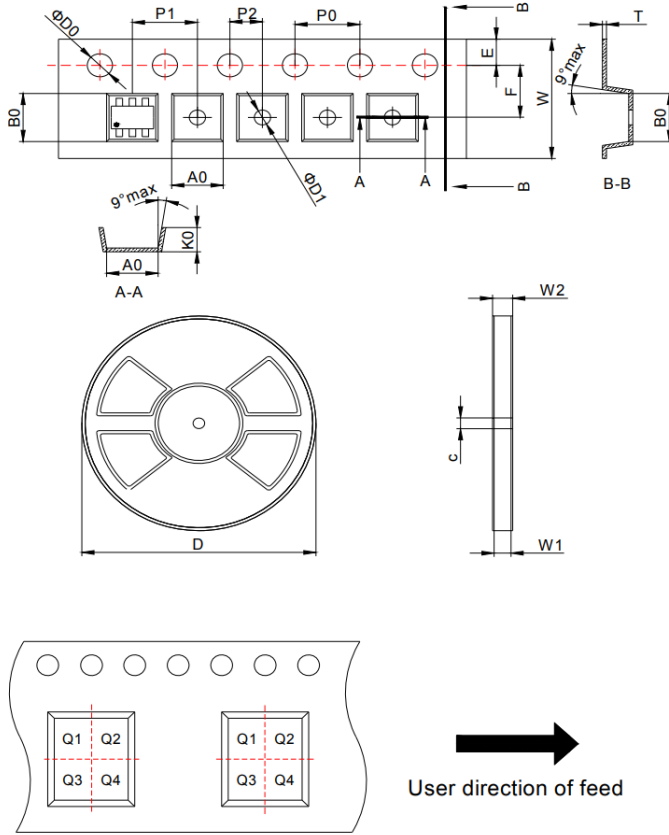
Pin 1 quadrant: Q3
