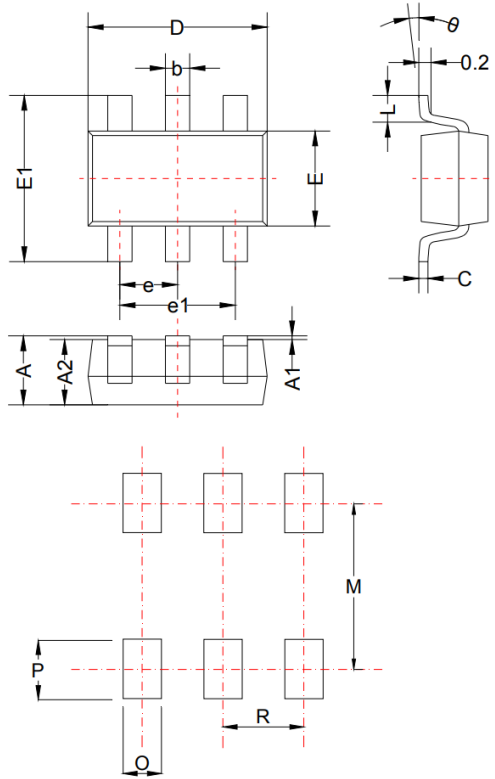
Recommended solder pad layout
